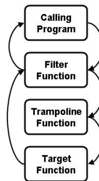
Figure 2: API Interception
