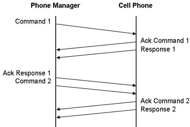
Figure 3: FBUS Communication
