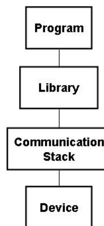
Figure 1: Filter Placement
