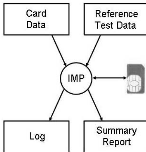
Figure 6: IMP Overview
